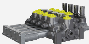
MA-D4 sectional series directional control valve block
